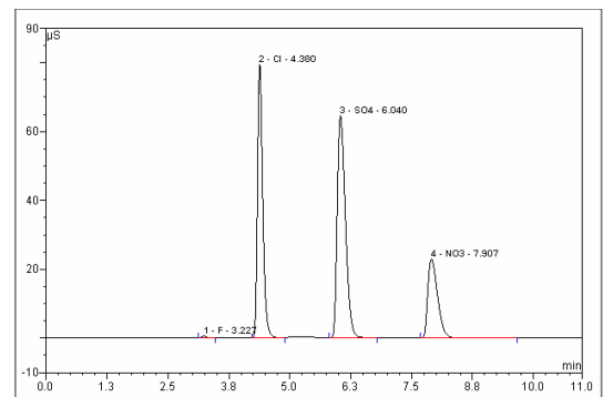
Figure 15. Anion chromatogram for sample D (North)
