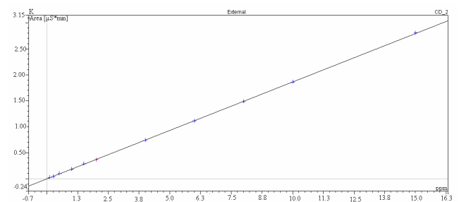
Figure 6. Calibration curves for K + determination
