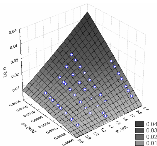
Figure 4. Dependence of the disequilibrium voltage U on the gas flow rate q_m and heating power P
