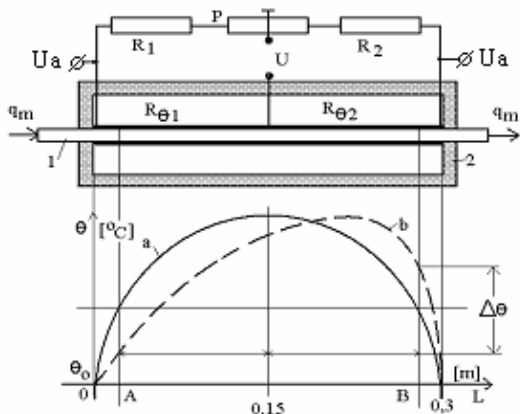
Figure 1. Operation principle of the electrothermal gas micro-flow meter
