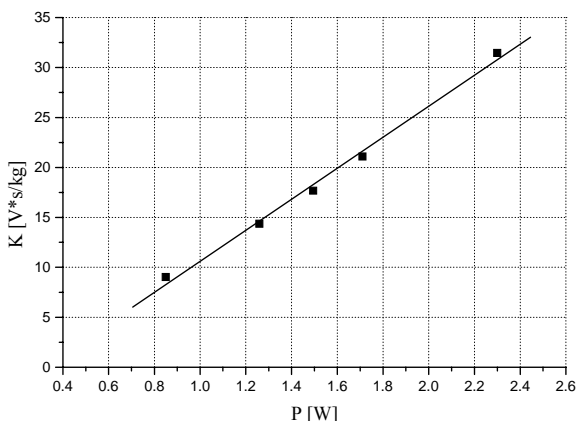
Figure 3. The interdependence between the apparatus sensitivity K and the heating power P
