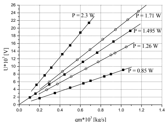
Figure 2. The static behaviour of the electrothermal gas micro-flowmeter
