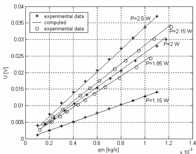
Figure 7. The simulation of static behaviour of the electrothermal micro-flowmeter
