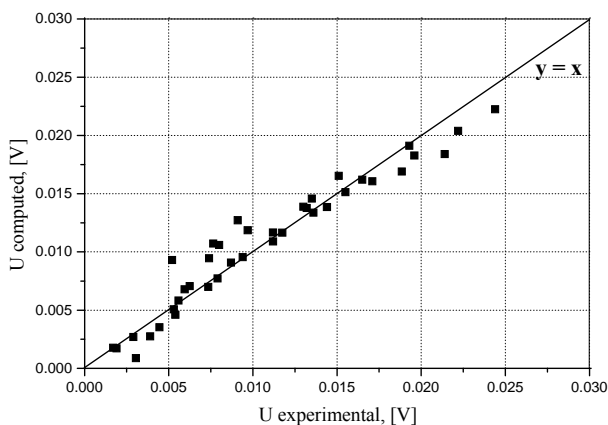
Figure 5. Correlation between the experimental results and the results obtained based on the mathematical model – for equation (5)
