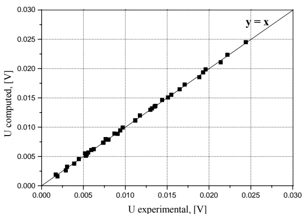
Figure 6. Correlation between the experimental results and the results obtained based on the mathematical model – for equation (6)
